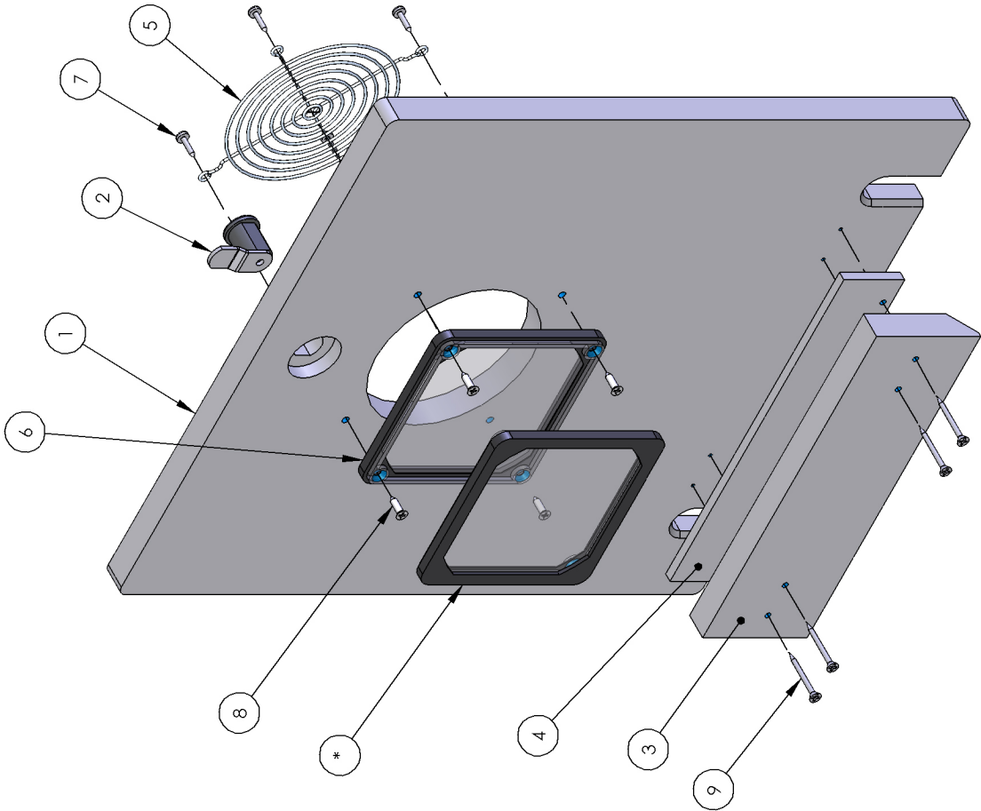
EXPLODED VIEW
